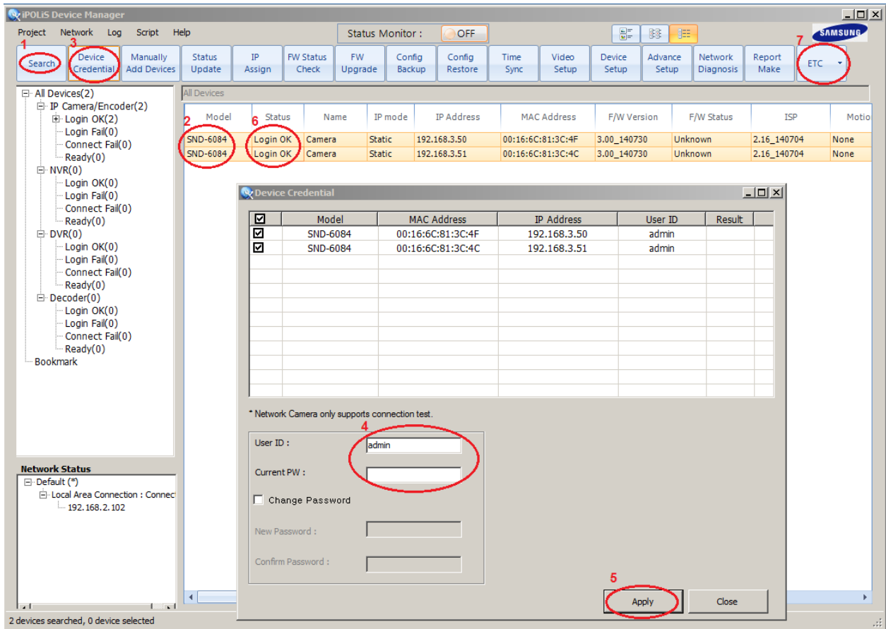
Figure 3: Insert camera credentials
