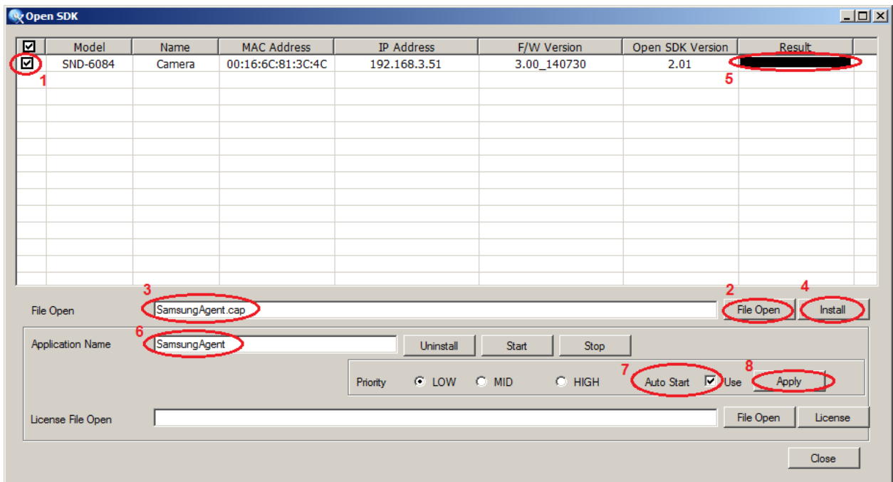
Figure 4: Open SDK configuration
